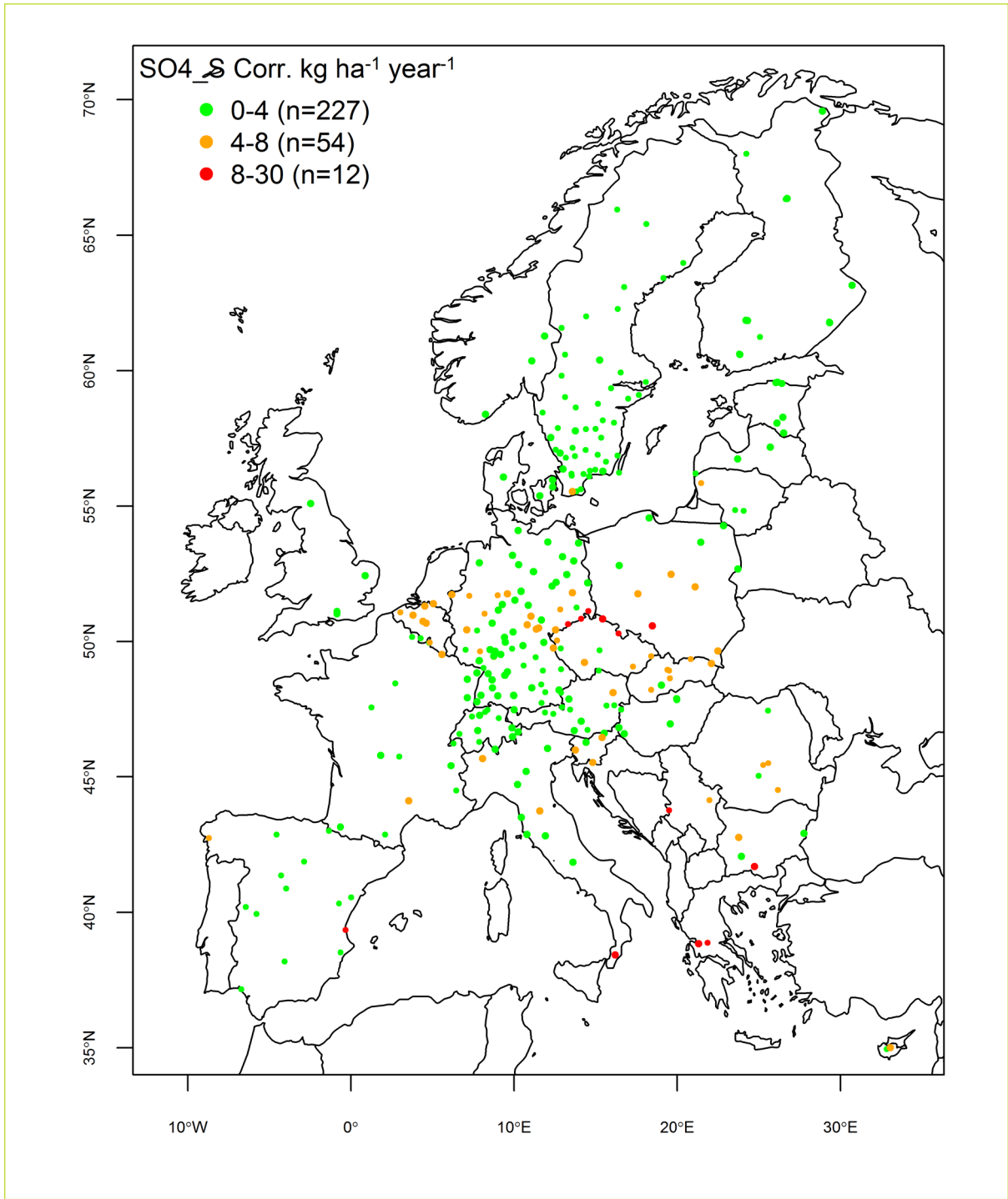
Figure 2.1-1: Sea-salt corrected annual throughfall deposition of sulphate-sulphur (SO 4 2- -S; kg S ha -1 year -1 ), 2016
