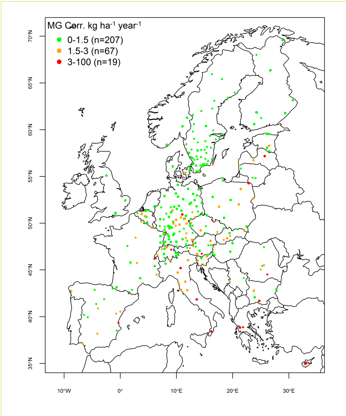
Figure 2.1-5: Sea-salt corrected annual throughfall deposition of magnesium ( Mg^{2+} ; kg\ ha^{-1}\ year^{-1} ), 2016
