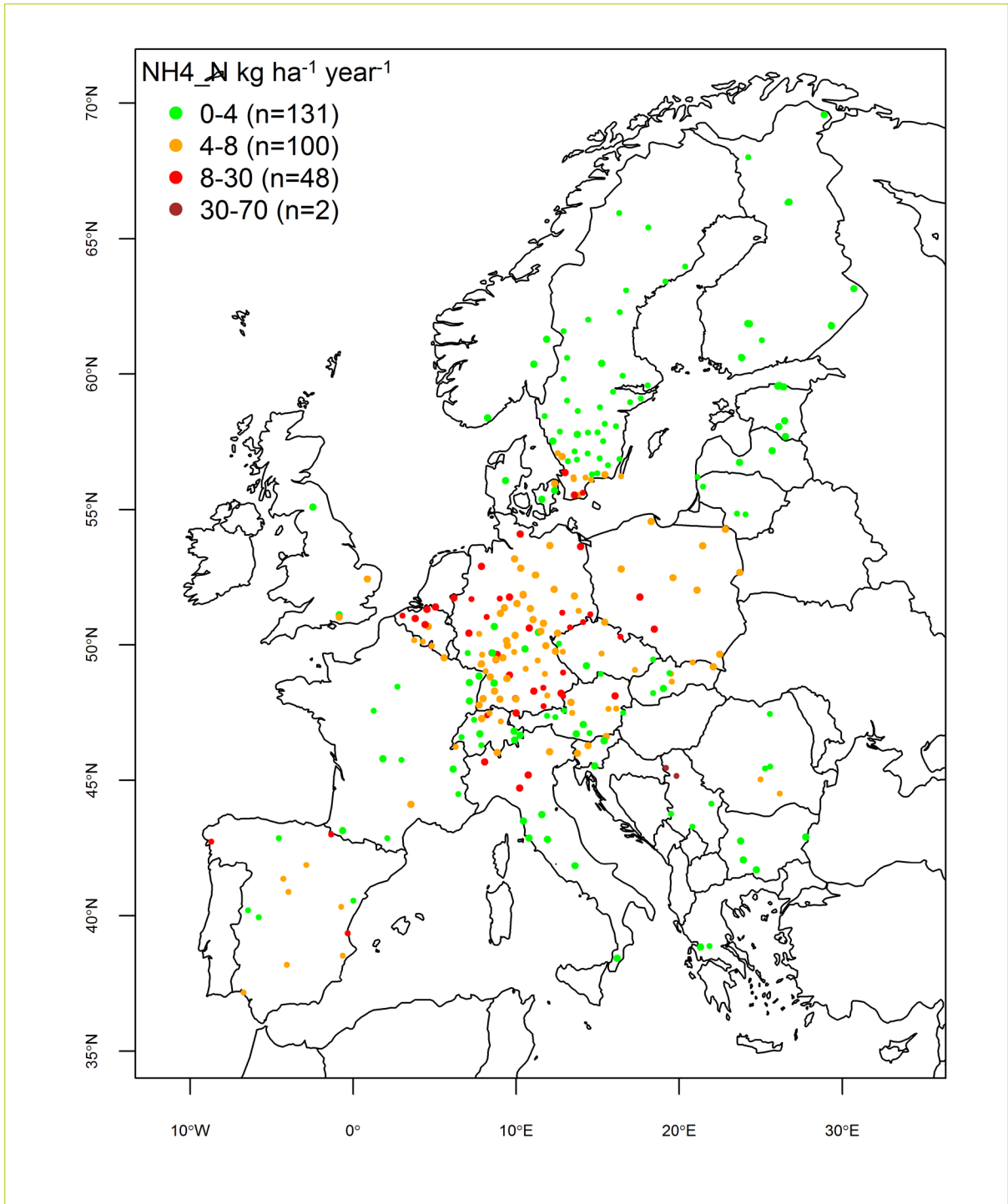
Figure 2.1-3: Annual throughfall deposition of ammonium-nitrogen (NH 4 + -N; kg N ha -1 year -1 ), 2016
