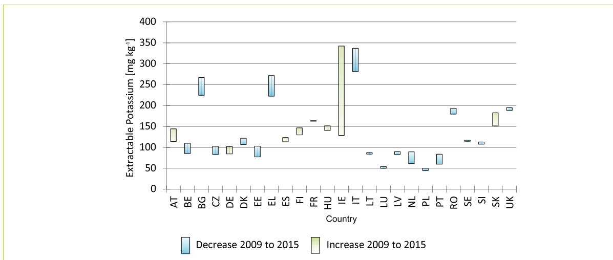
Figure 2.2-12: Change in extractable potassium in forest soils (mg K kg -1 ) between LUCAS Soil 2009/2012 and 2015, by country
